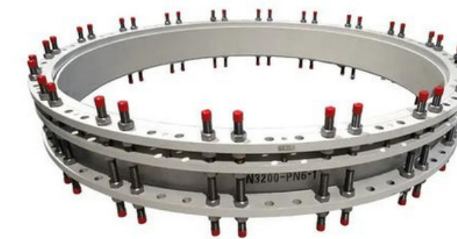
Dismantling Joint
